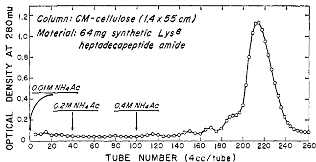
Figure 3. Carboxymethylcellulose chromatography of crude lysine 8 - \alpha^{1-17}\text{NH}_2 -ACTH. The material was applied to the column in 0.01 M ammonium acetate buffer of pH 4.5. After 40 aliquots (4 cc/tube) has been collected, a pH and concentration gradient was started by introducing a 0.2 M ammonium acetate solution (pH 6.7) into the column through a mixing chamber containing 500 cc of the starting buffer. When a total of 100 aliquots of eluate had been collected, the gradient was further increased by introducing a 0.4 M ammonium acetate solution through the mixing chamber for the remainder of the experiment.
