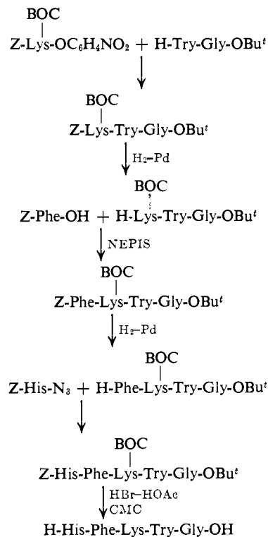
Figure 4. Synthetic scheme for lysine 8 - \alpha^{6-10} -ACTH.
